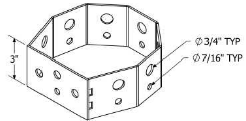
SCB 7 LINE CLUSTER BRACKET WEIGHT: 2 LBS
